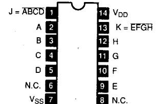
NTE4012B 14-Lead DIP, See Diag. 247 Dual 4-Input NAND Gate
