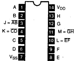
NTE4011B 14-Lead DIP, See Diag. 247 Quad 2-Input NAND Gate
