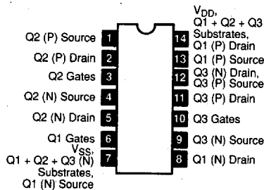
NTE4007 14-Lead DIP, See Diag. 247 Dual Complementary Pair Plus Inverter
