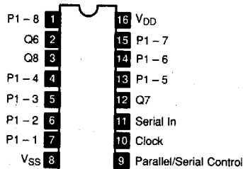
NTE4014B 16-Lead DIP, See Diag. 249 8-Stage Shift Register Synchronous Parallel or Serial Input/Serial Output
