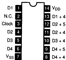
NTE4006B 14-Lead DIP, See Diag. 247 18-Stage Static Shift Register
