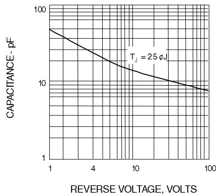
Fig. 4-TYPICAL JUNCTION CAPACITANCE
