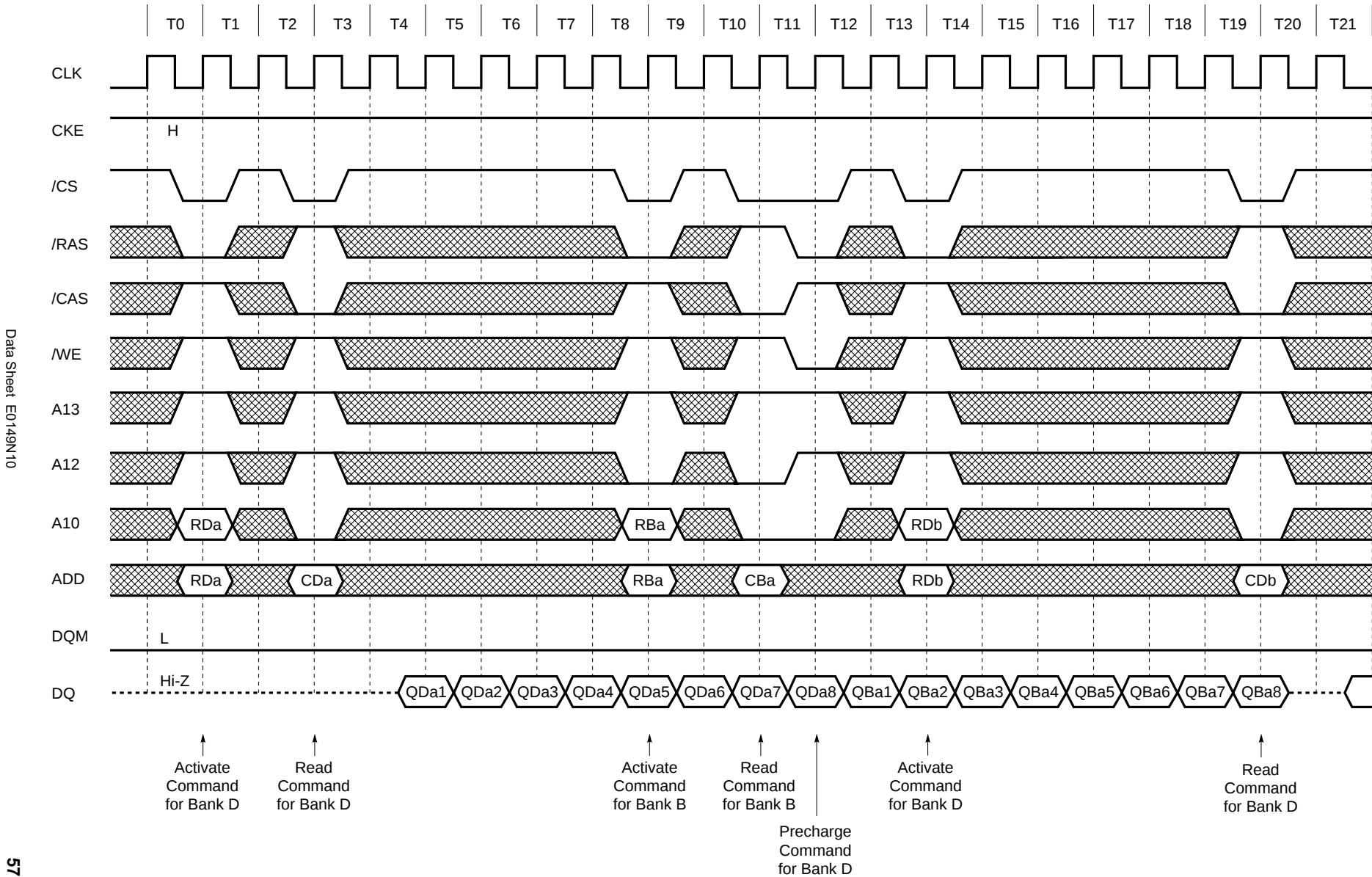
13.14 Random Row Read (Ping-Pong Banks) (1/2) (Burst Length = 8, /CAS Latency = 2)
