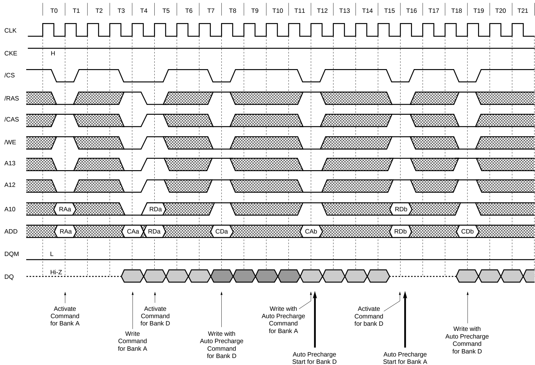
Auto Precharge after Write Burst (2/2) (Burst Length = 4, ICAS Latency = 3)
