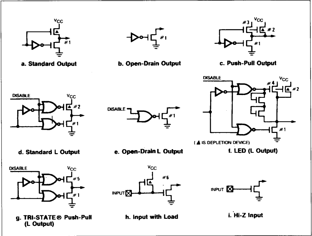
Figure 5 : Output Configurations.
