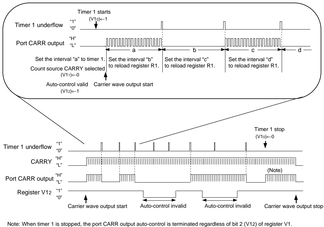
Fig. 14 Port CARR output control by timer 1
