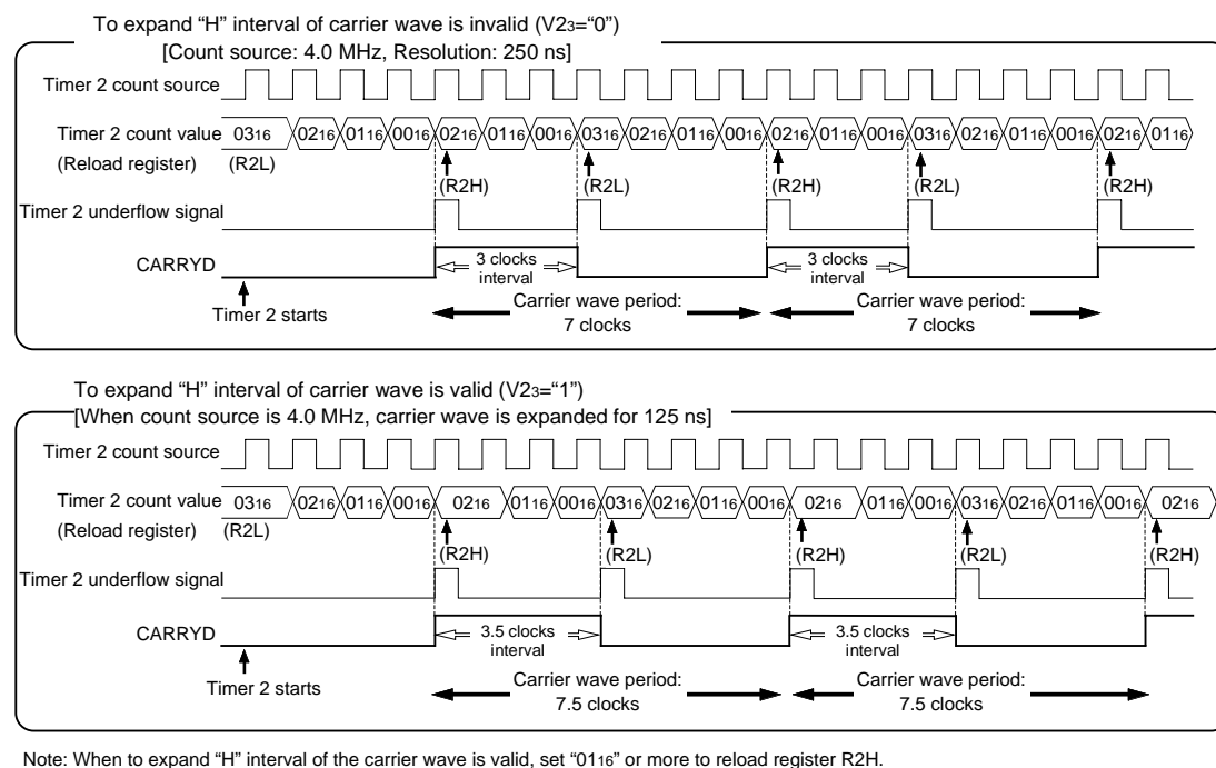
Fig. 15 Carrier wave generation example by timer 2
