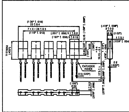
OUTLINE AND PIN CONNECTION
