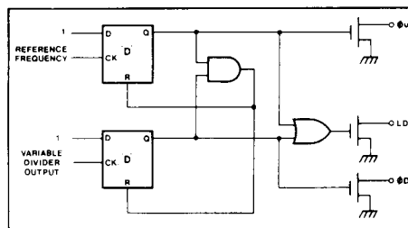
Fig.3 Logic diagram of phase frequency comparator
