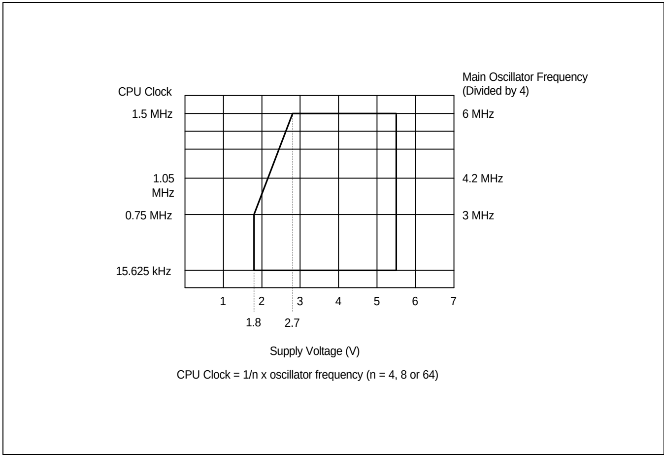
Figure 16-3. Standard Operating Voltage Range
