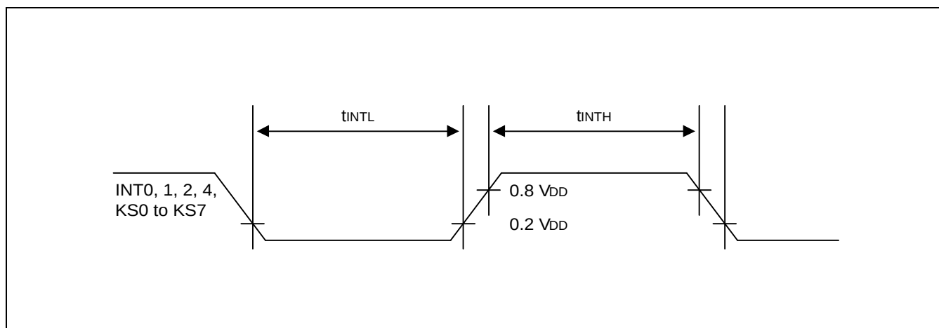
Figure 14-8. Input Timing for External Interrupts and Quasi-Interrupts
