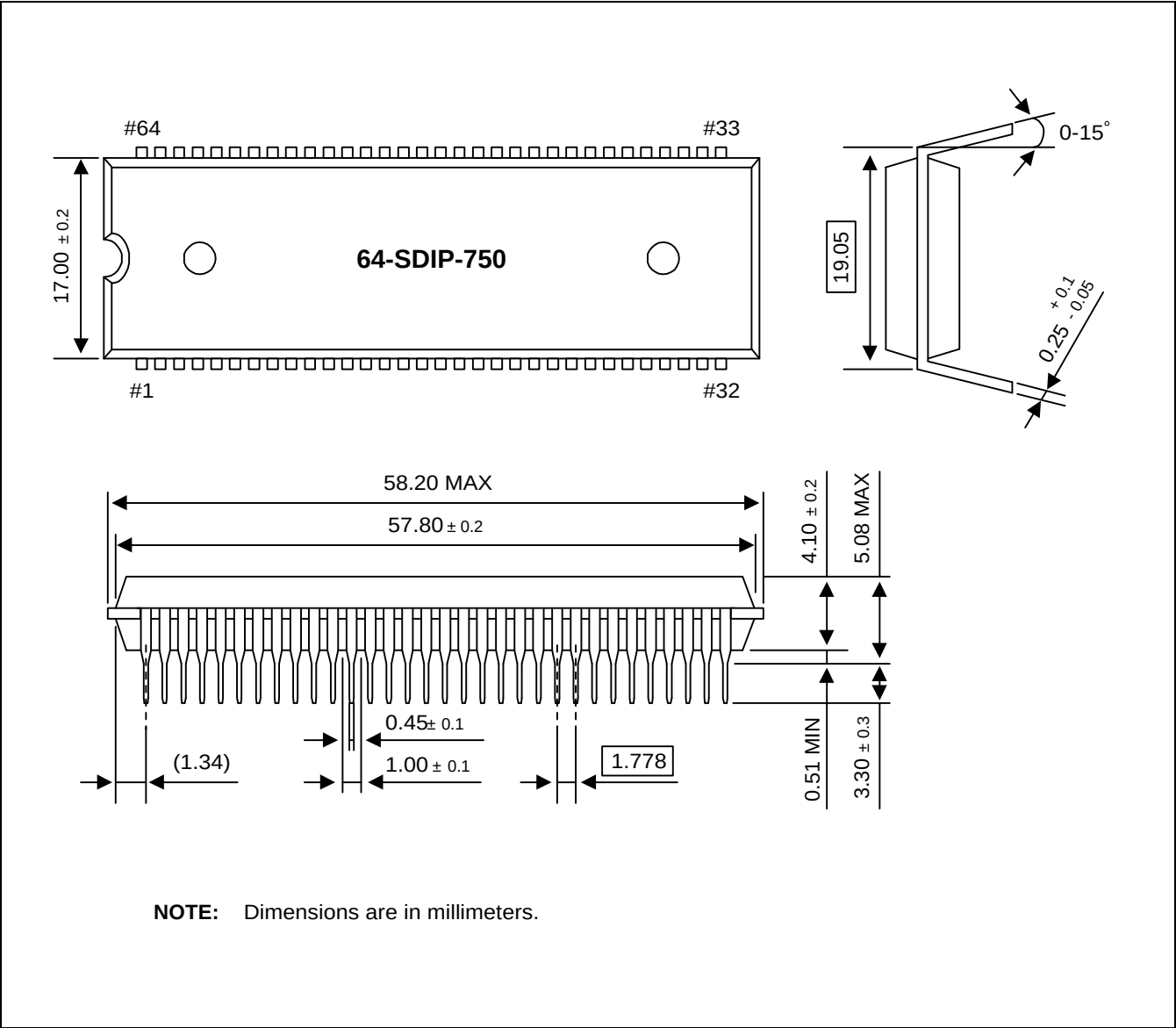
Figure 15-2. 64-SDIP-750C Package Dimensions
