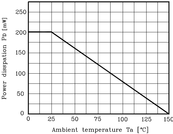
Fig.9 P_D - T_a
