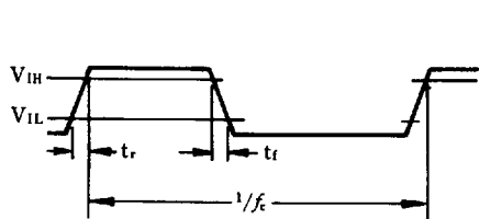
Fig. 4 Clock timing
