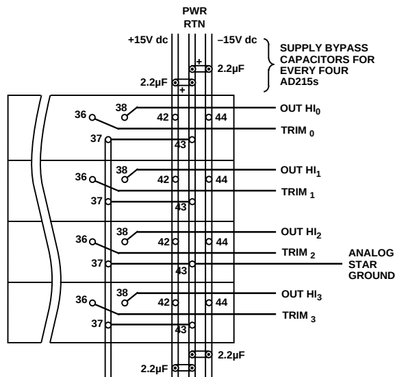
Figure 20a. PCB Layout for Unity Gain
