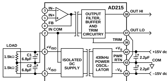
Figure 19. Using the Isolated Power Supplies
