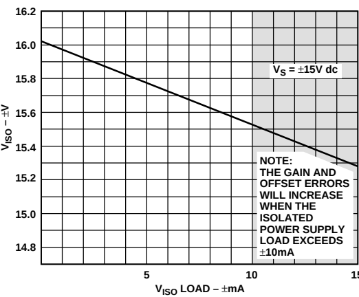
Figure 10. ±VISO Supply Voltage vs. Load
