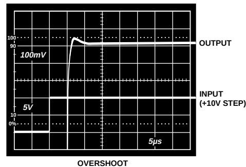
Figure 7a. Overshoot to a Full-Scale Step Input (G = 1 V/V)
