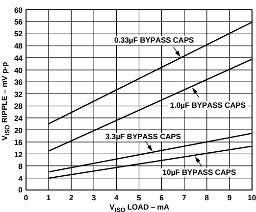
Figure 9. ±VISO Supply Ripple vs. Load
