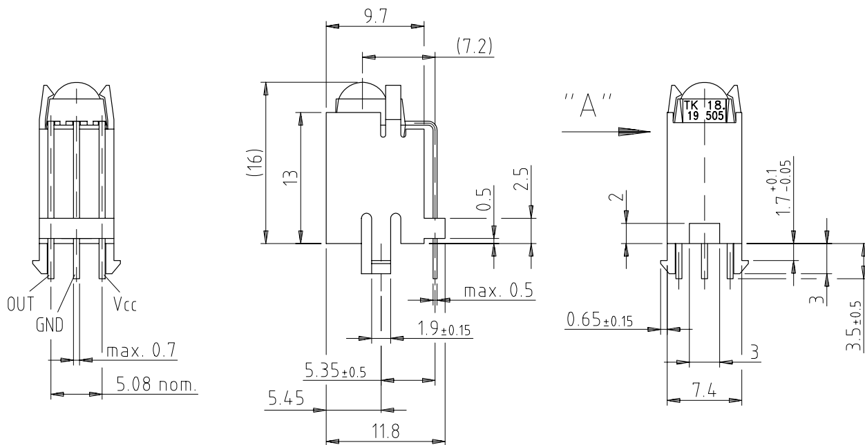
View "A"
