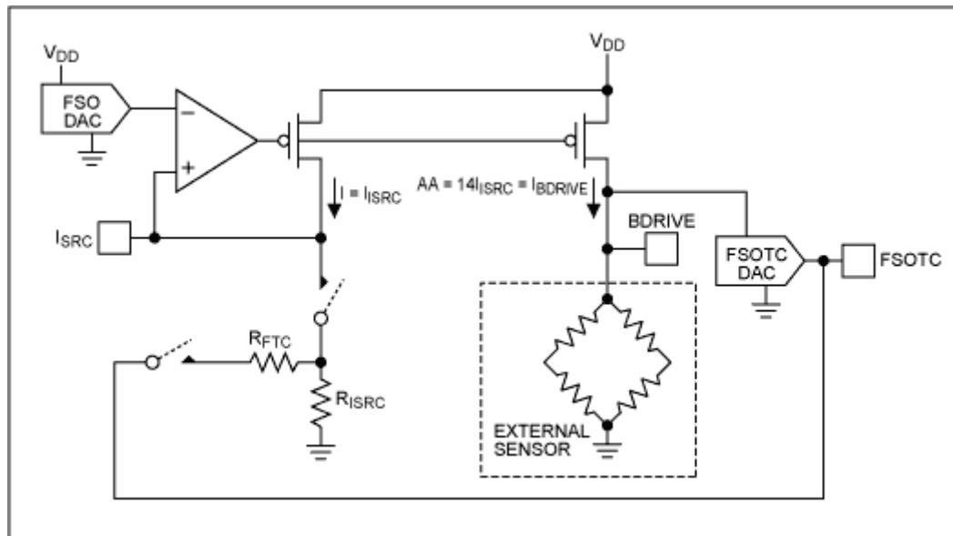
Figure 3a. Patented sensor-bridge excitation circuit
