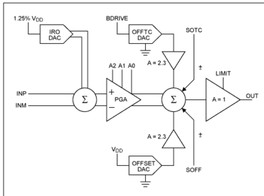
Figure 3b. A differential analog-output path
