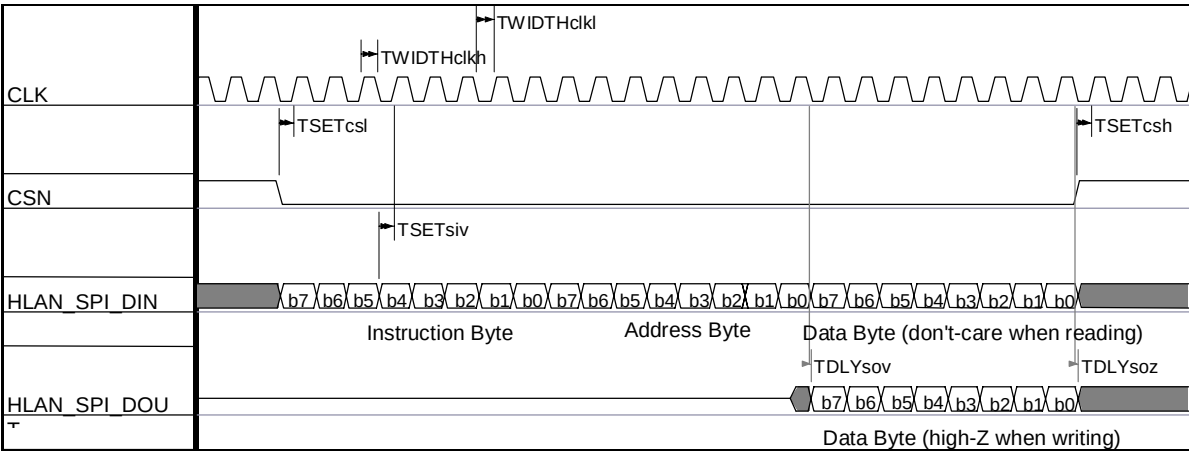
Figure 3. SPI Timing
