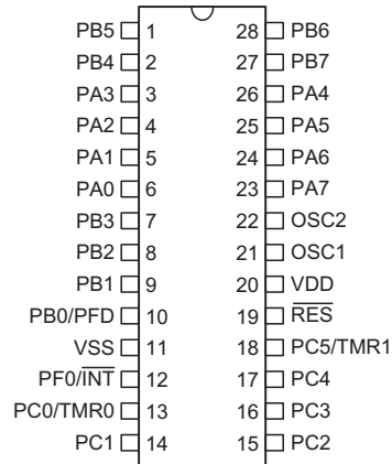
HT48RA3 – 28 SKDIP-A/SOP-A
