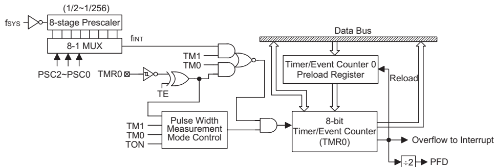
Timer/Event Counter 0
