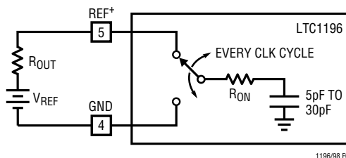
Figure 9. Reference Input Equivalent Circuit
