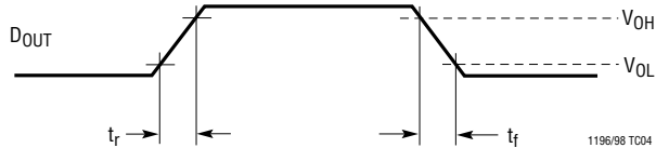
Voltage Waveform for D_{OUT} Rise and Fall Times, t_r , t_f
