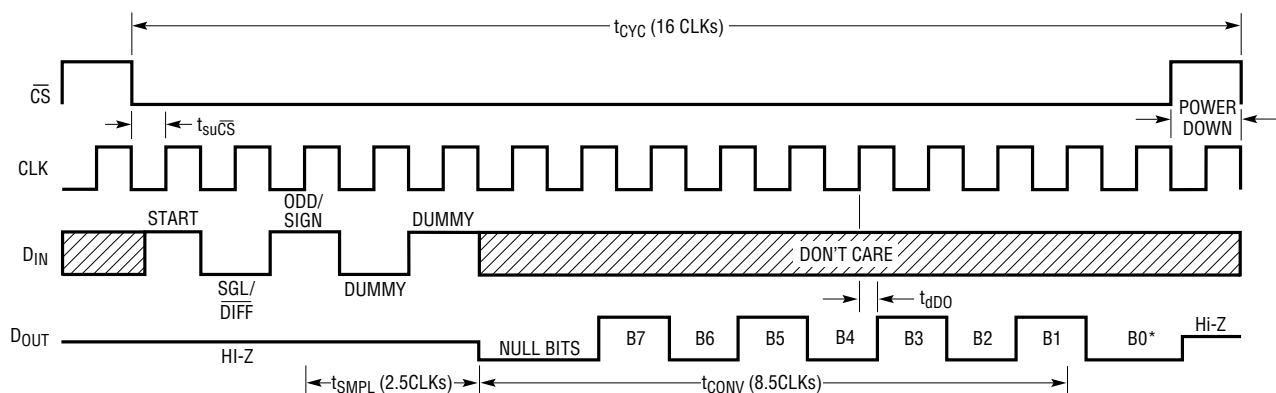
Figure 1. LTC1196 Operating Sequence
