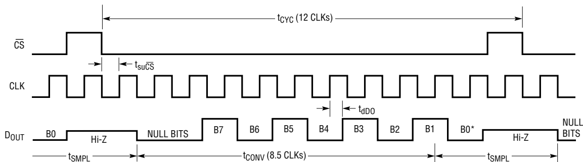
Figure 1. LTC1196 Operating Sequence
