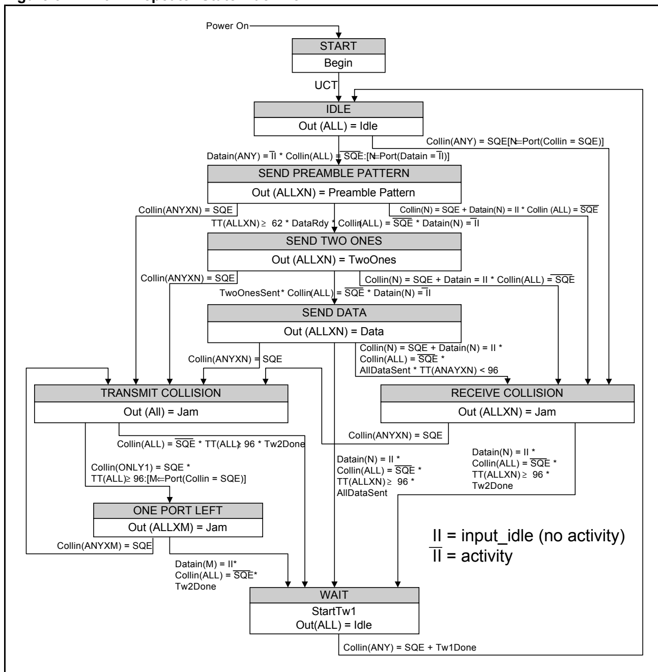
Figure 3: LXT917 Repeater State Machine
