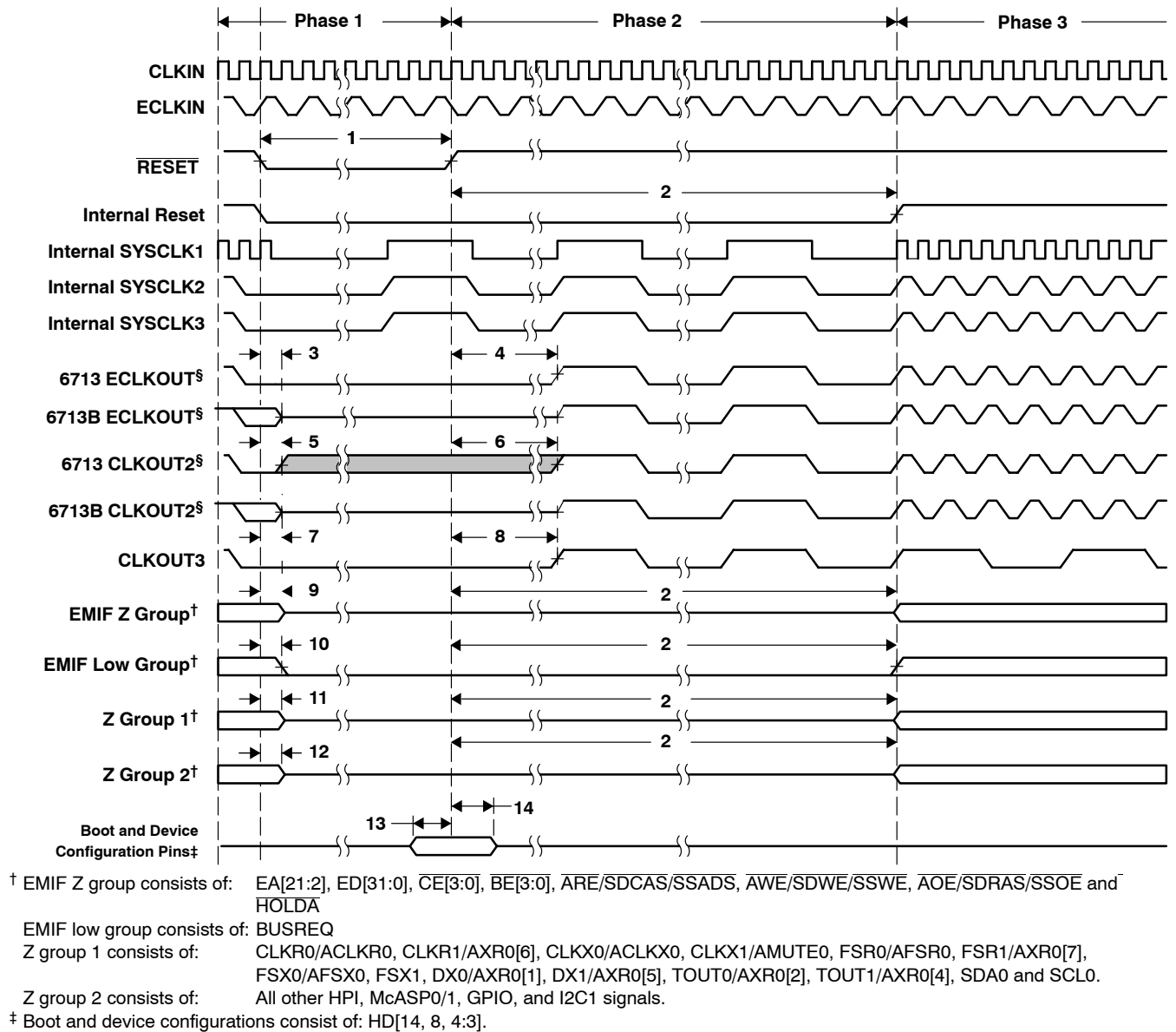
Figure 47. Reset Timing
