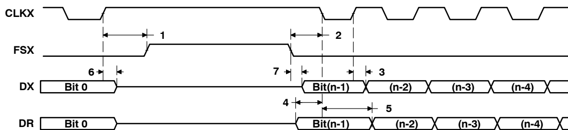
Figure 62. McBSP Timing as SPI Master or Slave: CLKSTP = 11b, CLKXP = 1
