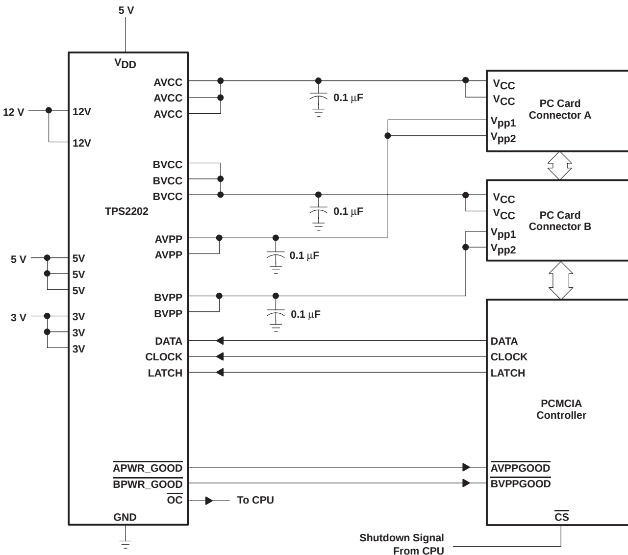
Figure 25. Detailed Interconnections and Capacitor Recommendations
