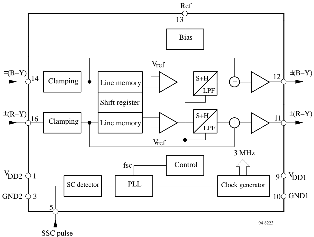
Figure 1. Block diagram
