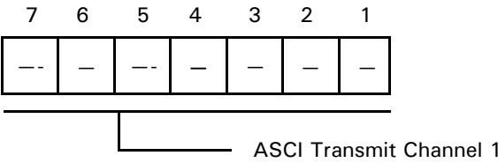
Figure 29. ASCII Register
