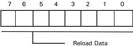
Figure 45. Timer Data Register
