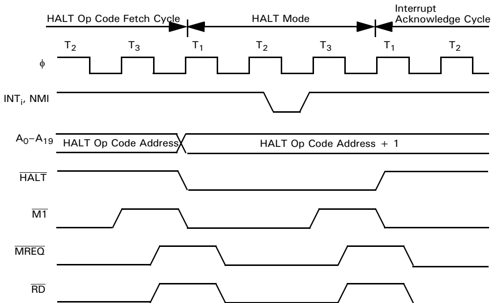
Figure 13. HALT Timing
