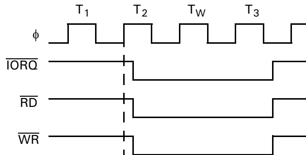
Figure 12. I/O READ and WRITE Cycles with \overline{IOE} = 0
