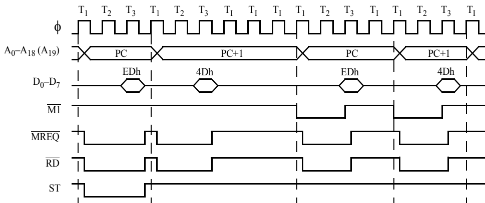
Figure 77. RETI Instruction Sequence with \overline{MIE}=0
