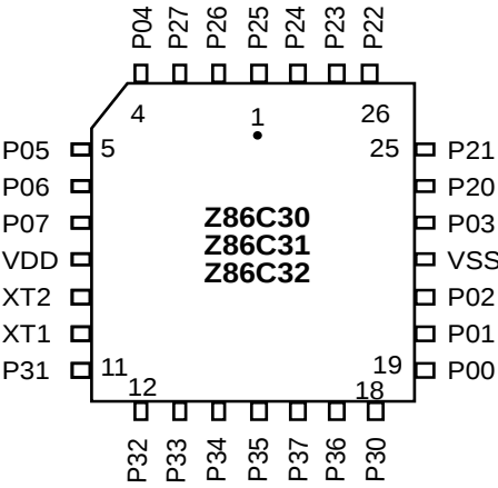
28-Pin PLCC Configuration
