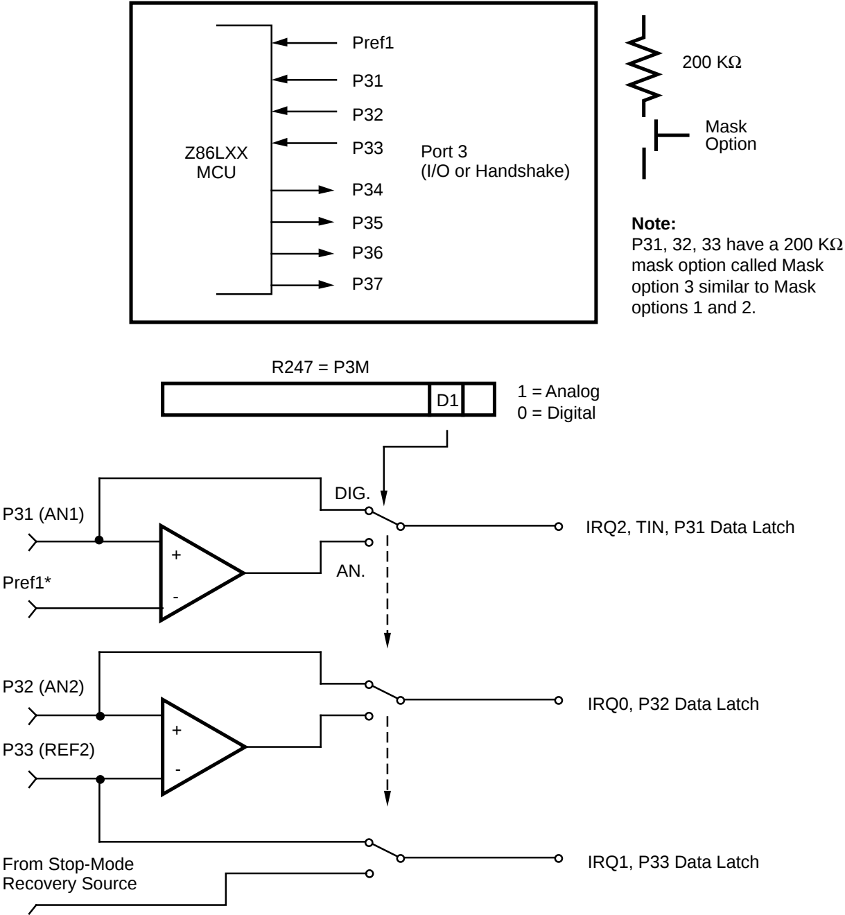
Figure 12. Port 3 Configuration
