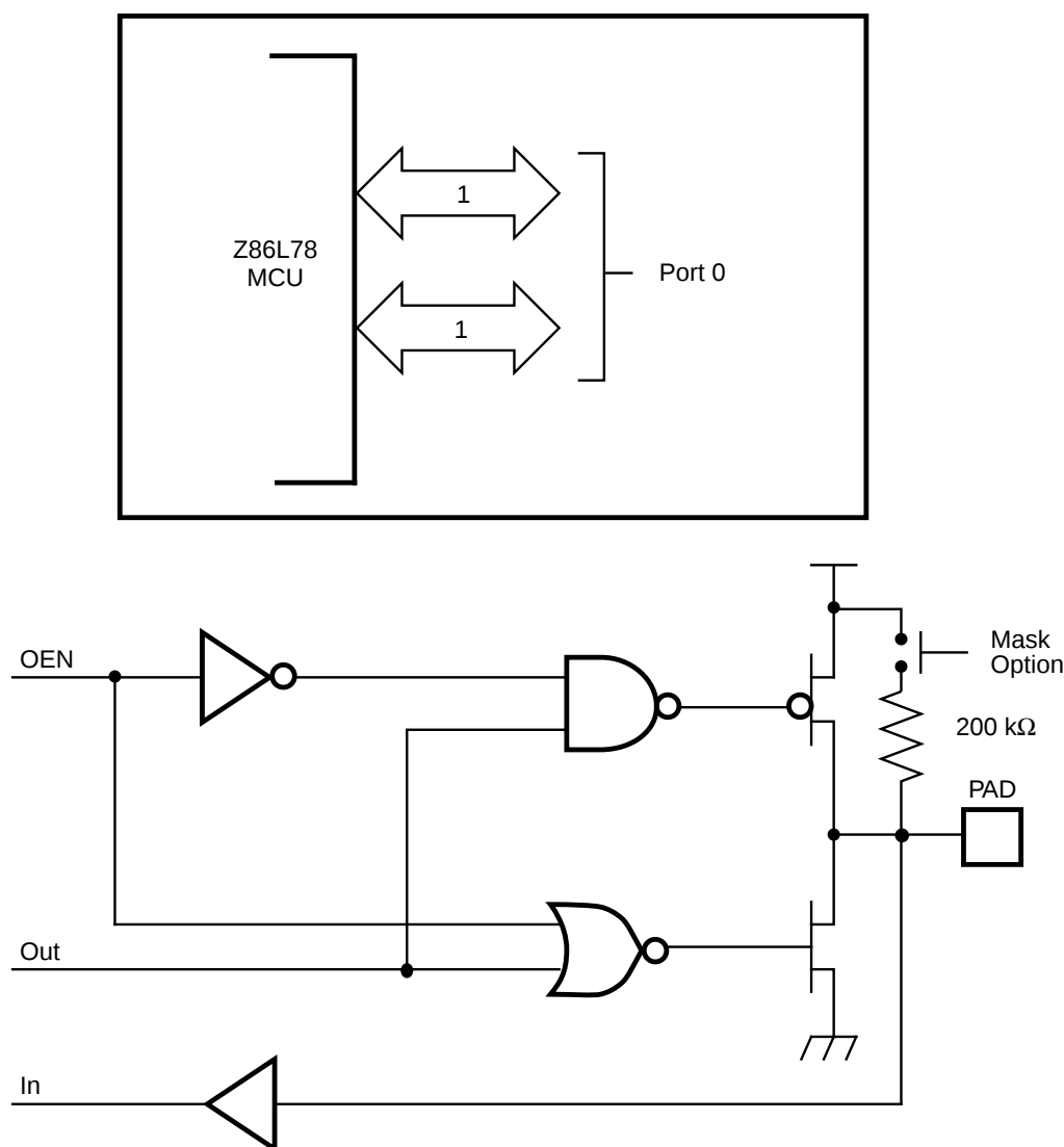
Figure 9. Port 0 Configuration
