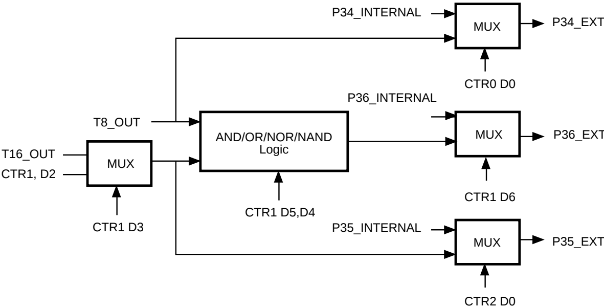
Figure 29. Output Circuit
