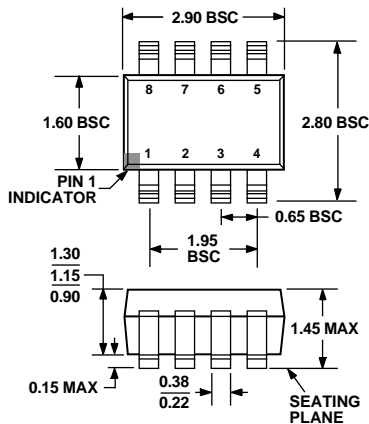
Figure 53. 8-Lead Small Outline Transistor Package [SOT-23] (RJ-8)
