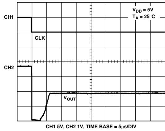
Figure 20. Exiting Power-Down
