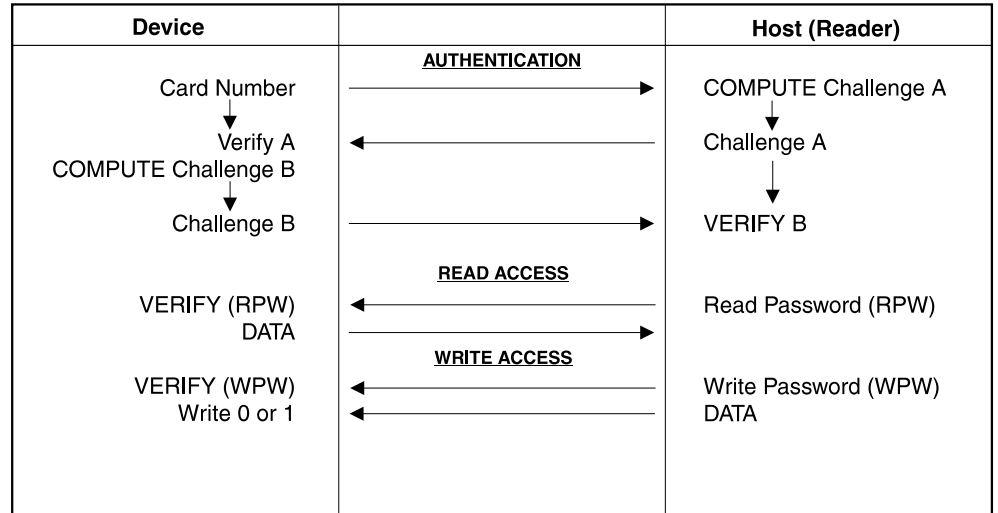
Figure 2. Security Methodology
