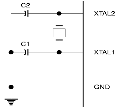
Figure 1. Oscillator Connections
