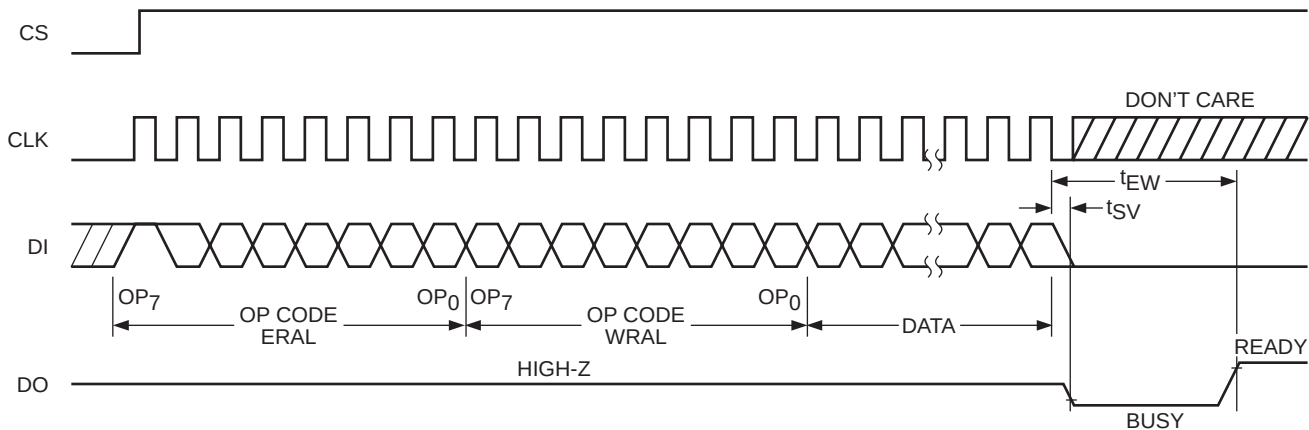
Figure 12. WRAL Timing
