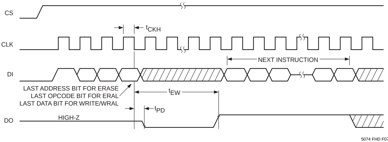
Figure 5. Program/Erase Timing
