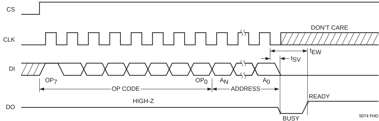
Figure 10. Erase Timing
