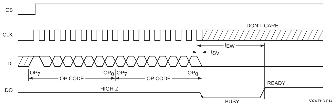
Figure 11. ERAL Timing
