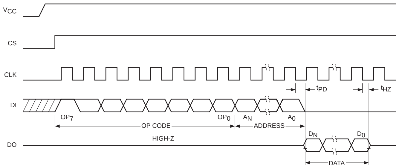
Figure 7. Read Timing
