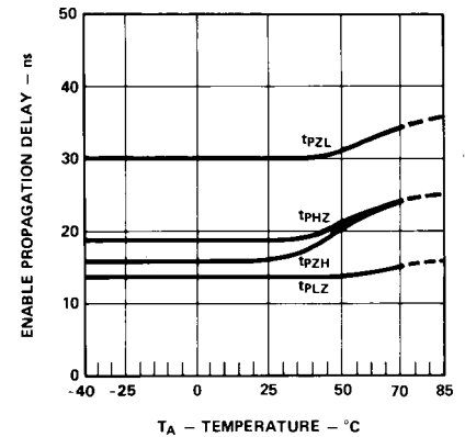
Figure 10. Typical Enable Propagation Delay vs. Ambient Temperature.
