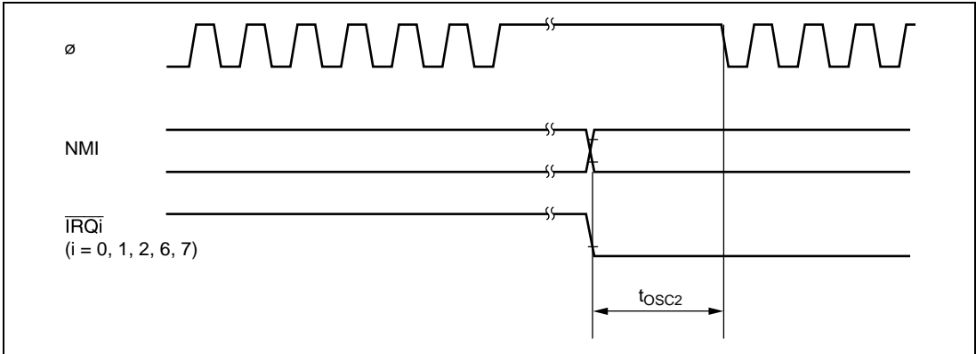
Figure 28.8 Oscillation Setting Timing (Exiting Software Standby Mode)
