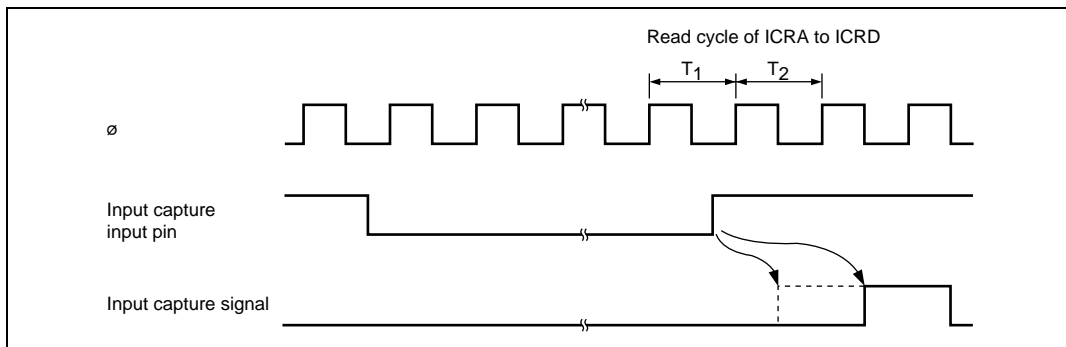
Figure 11.8 Input Capture Input Signal Timing (When ICRA to ICRD are Read)
