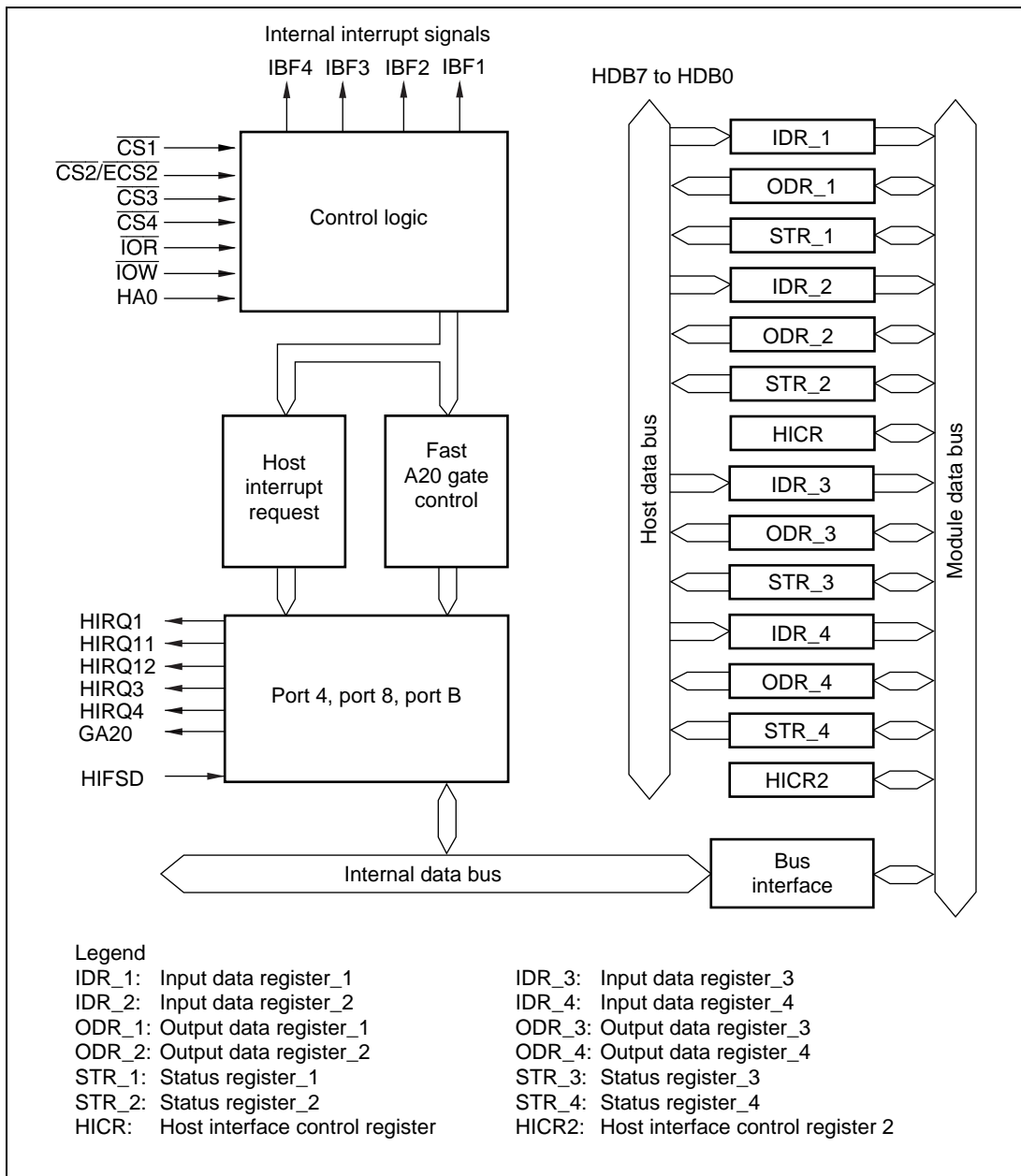
Figure 18.1 Block Diagram of XBS
