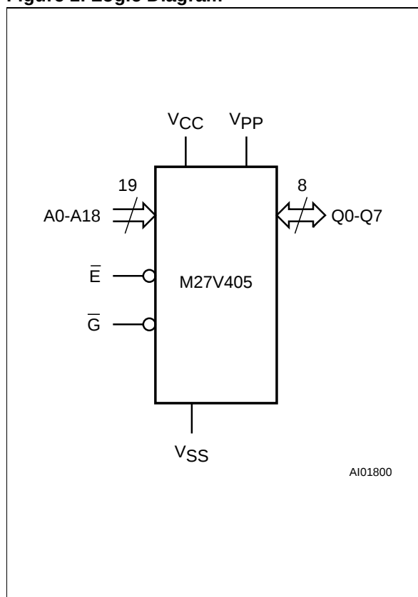
Figure 1. Logic Diagram
