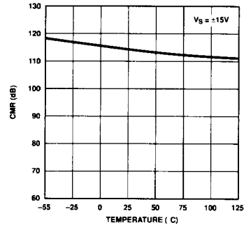
CMR vs TEMPERATURE
