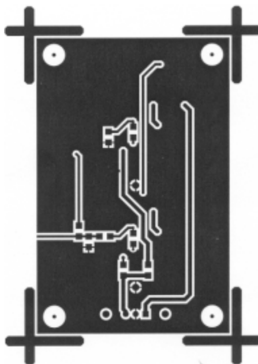
Figure 20. Evaluation Board Layout (Bottom)
