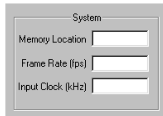
Figure 4: System Options
