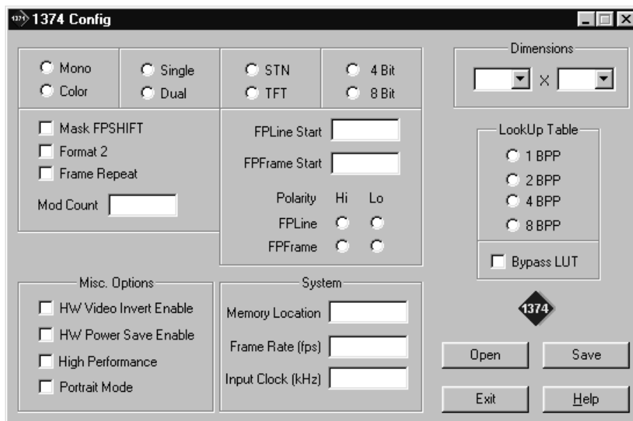
Figure 1: 1374CFG Window
