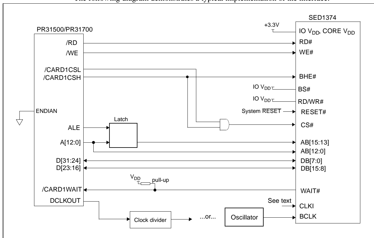
Figure 2-1: SED1374 to PR31500/PR31700 Direct Connection
