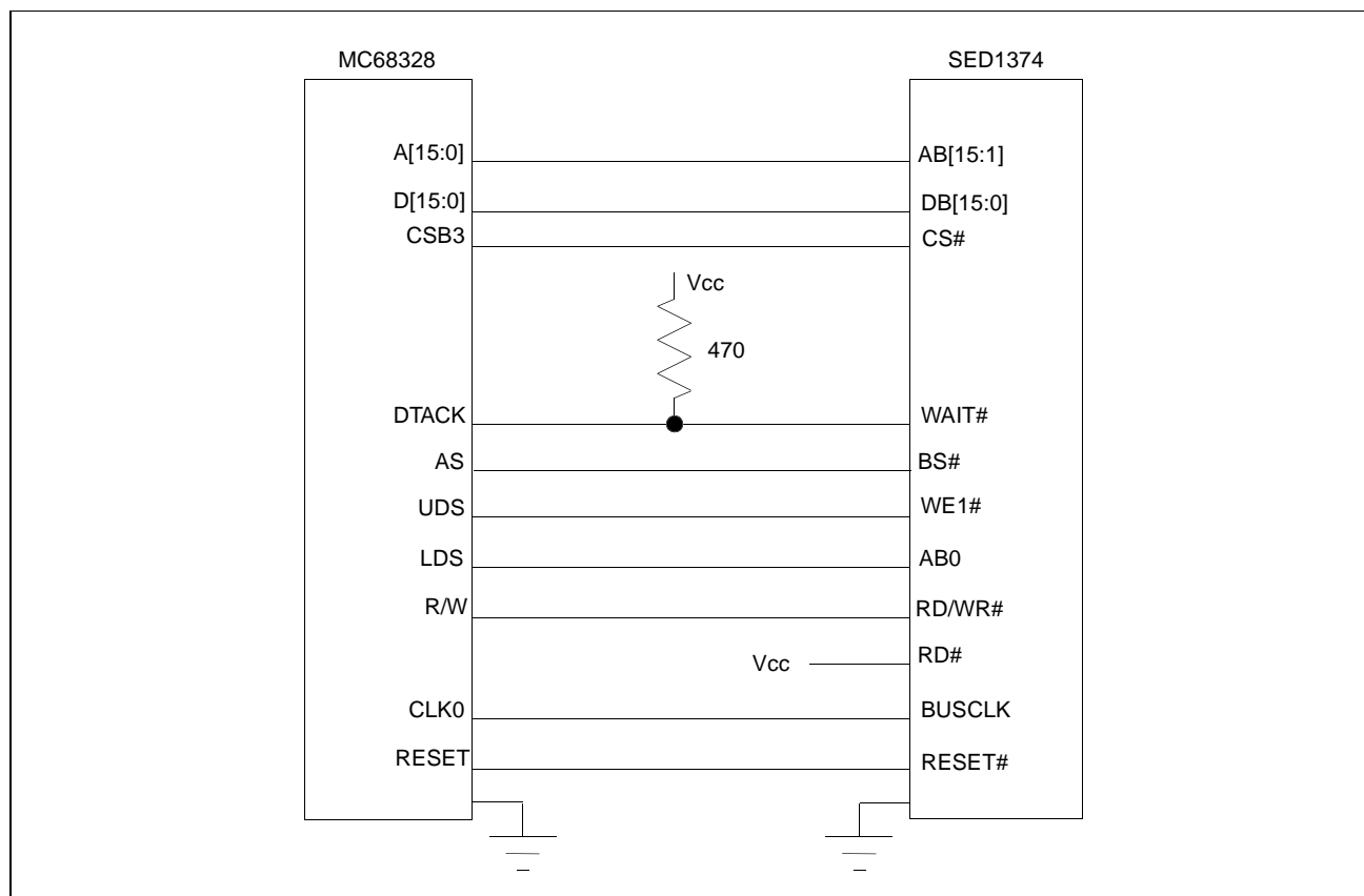
Figure 4-1: Typical Implementation of MC68328 to SED1374 Interface - MC68K #1
