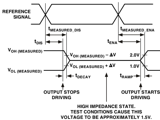
Figure 29. Output Enable/Disable
