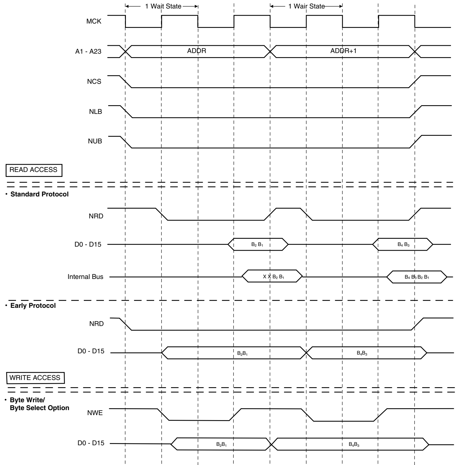
Figure 27. 1 Wait, 16-bit Bus Width, Word Transfer
