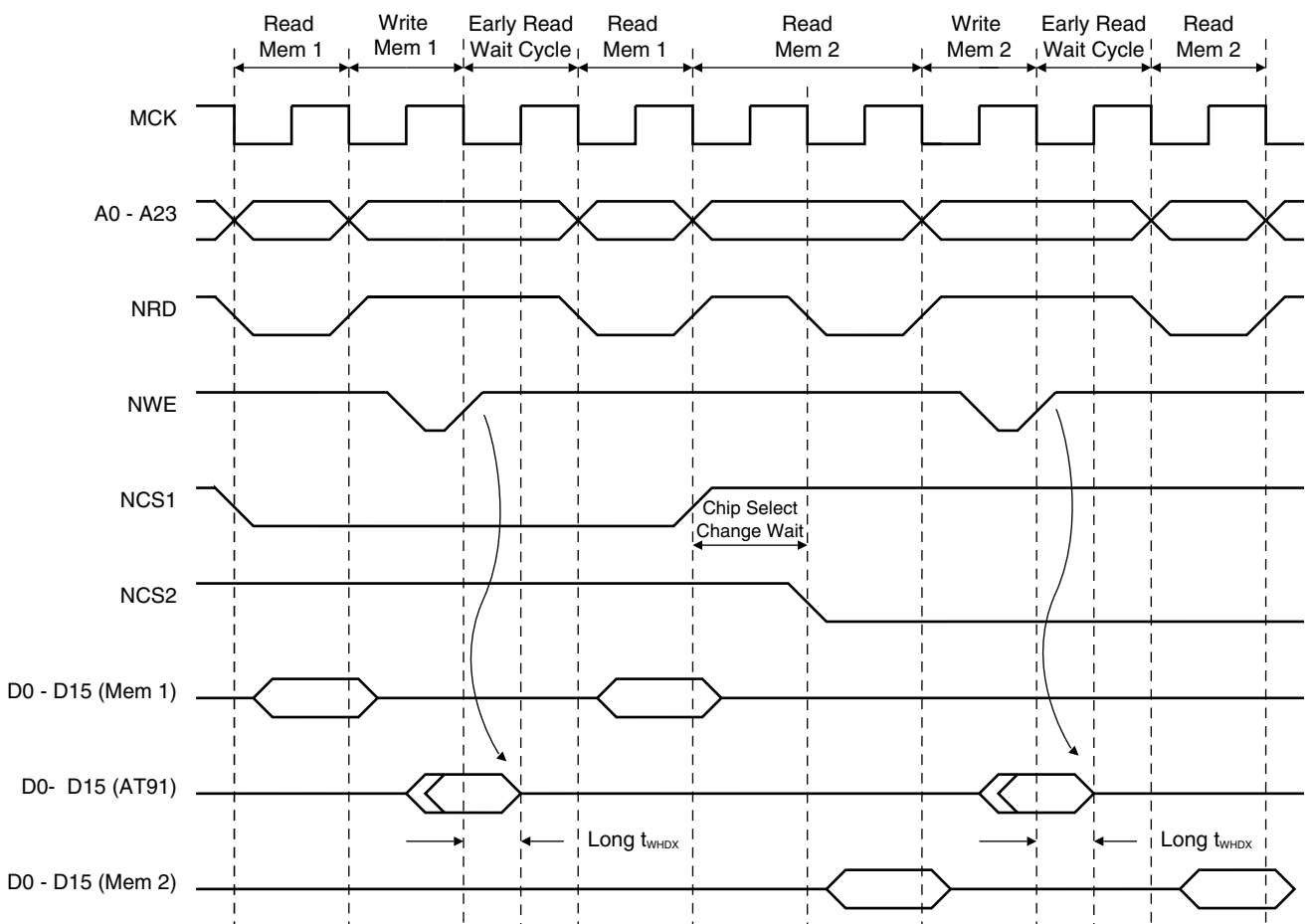
Figure 23. Early Read Protocol Without t_F
