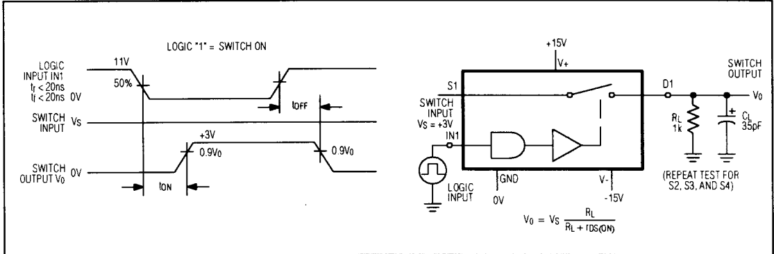
Figure 1. Switching-Time Test Circuit
