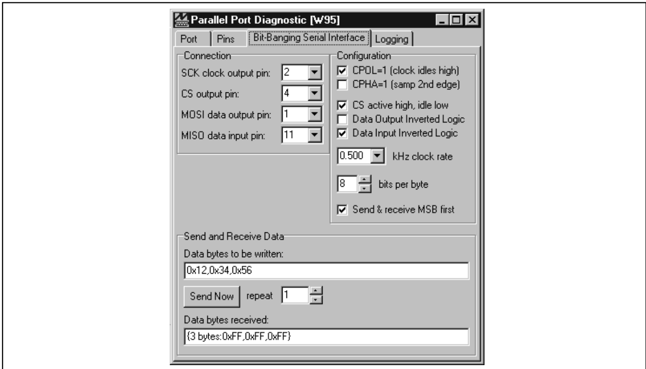
Figure 5. SPI/3-Wire Diagnostic
