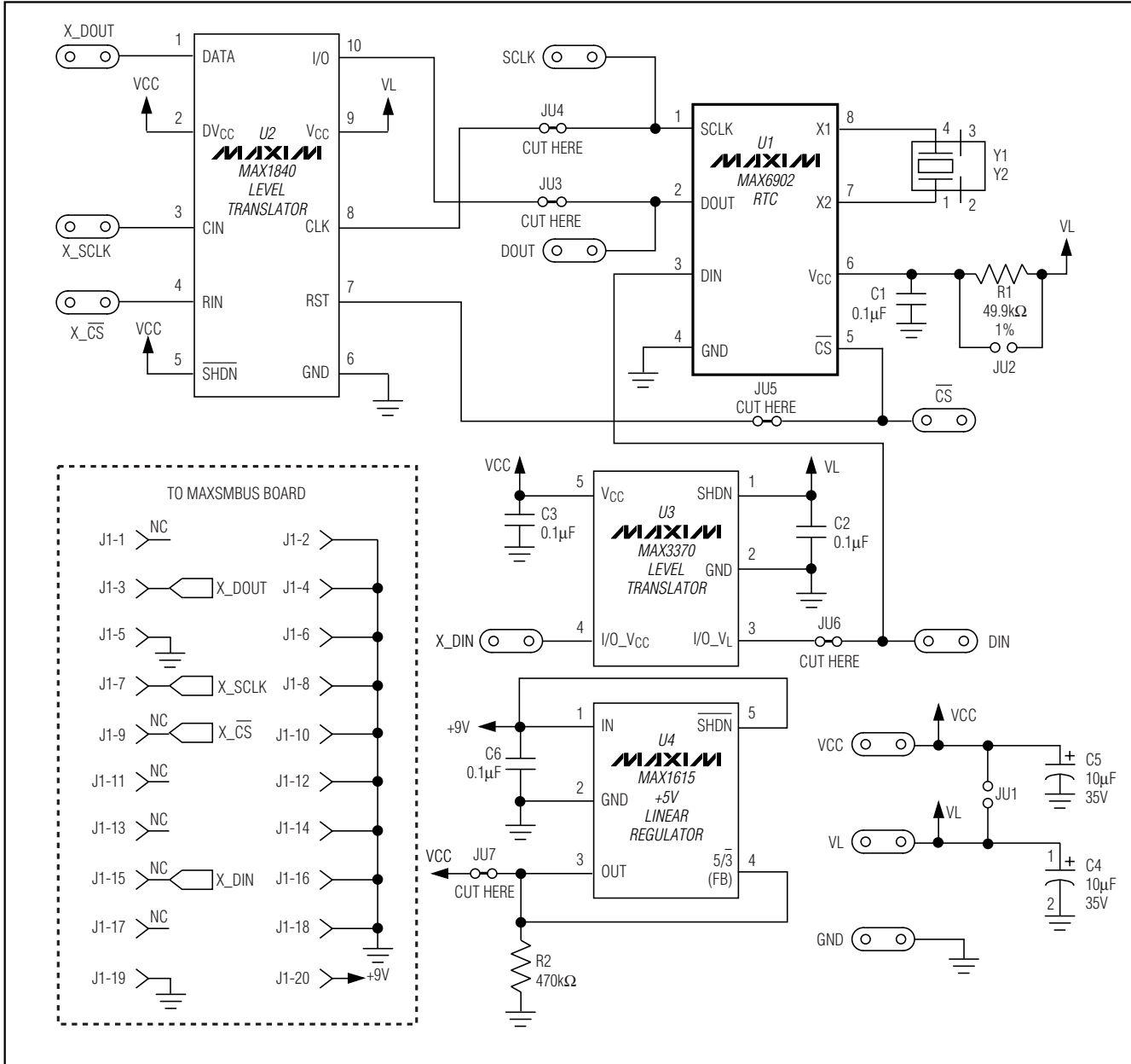
Figure 7. MAX6902 EV Kit Schematic
