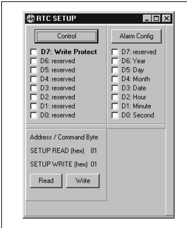
Figure 4. Setup Screen
