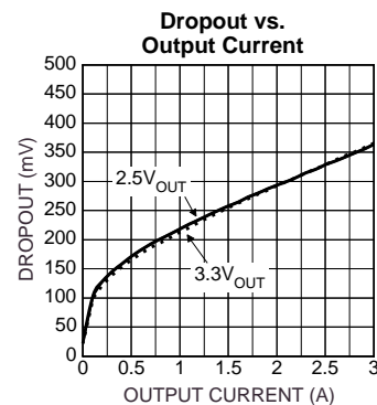
Adjustable Regulator
