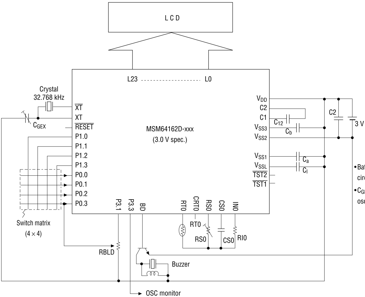
3.0 V Spec. Application Circuit
