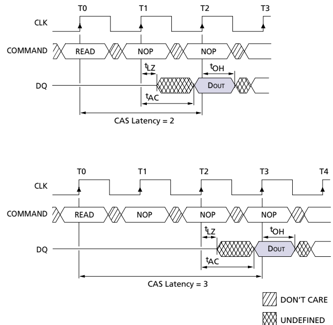
Figure 6 CAS Latency
