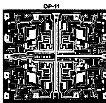
DIE SIZE 0.086 × 0.072 inch, 6192 sq. mils (2.18 × 1.83 mm, 3.99 sq. mm)
