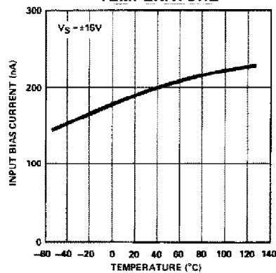
BIAS CURRENT vs TEMPERATURE
