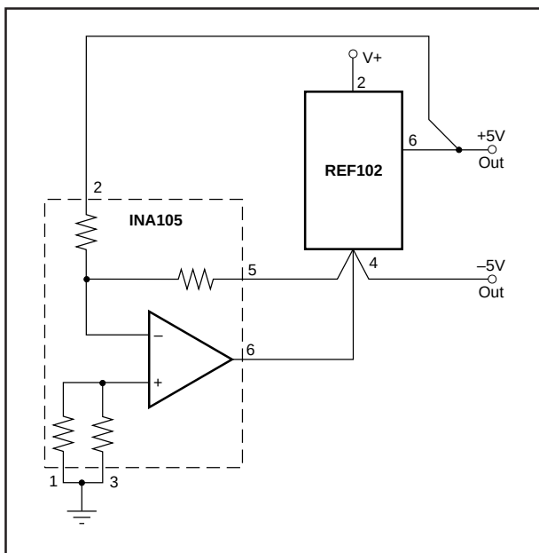
FIGURE 12. ±5V Reference.
