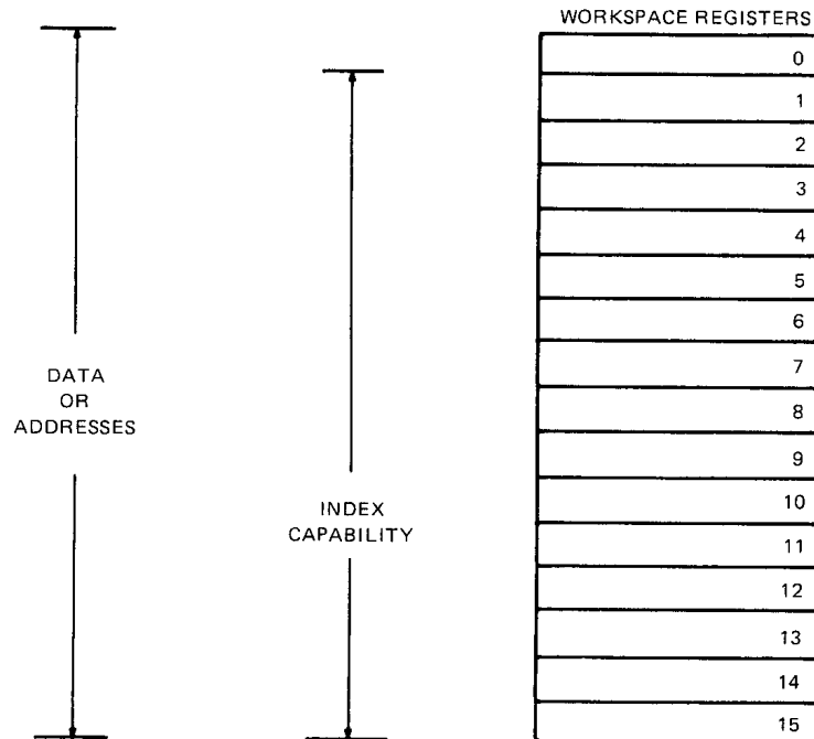
FIGURE 6 – WORKSPACE REGISTERS USABLE AS INDEX REGISTERS
