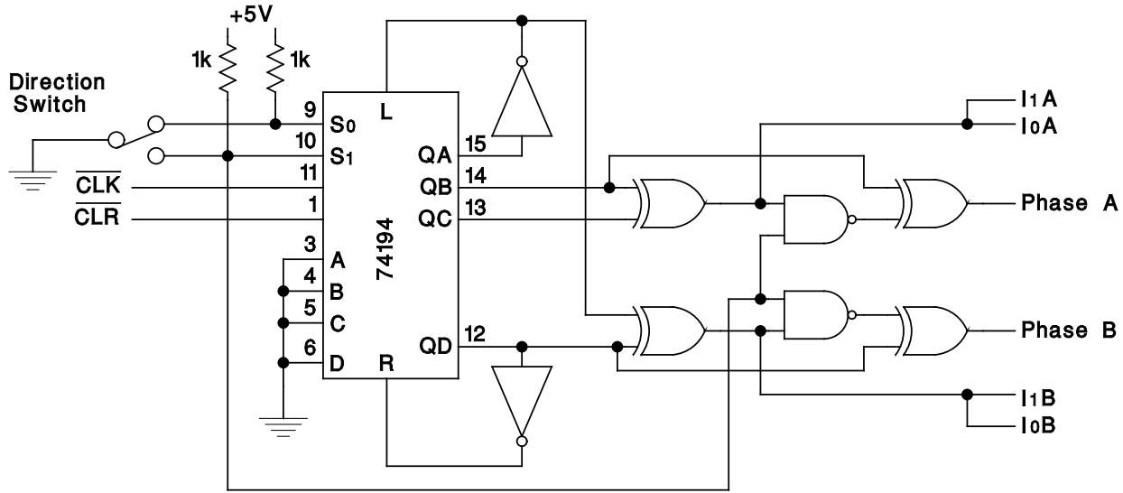
Figure 14: Half-Step, Bidirectional Drive Logic
