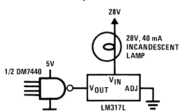
Fully Protected (Bulletproof) Lamp Driver
