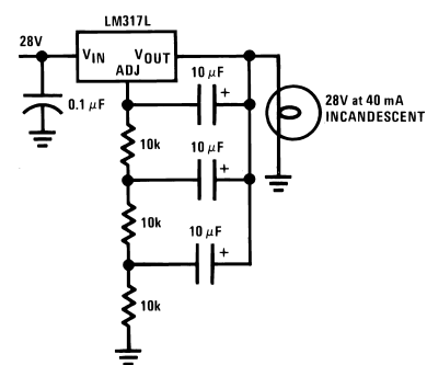
Lamp Flasher
