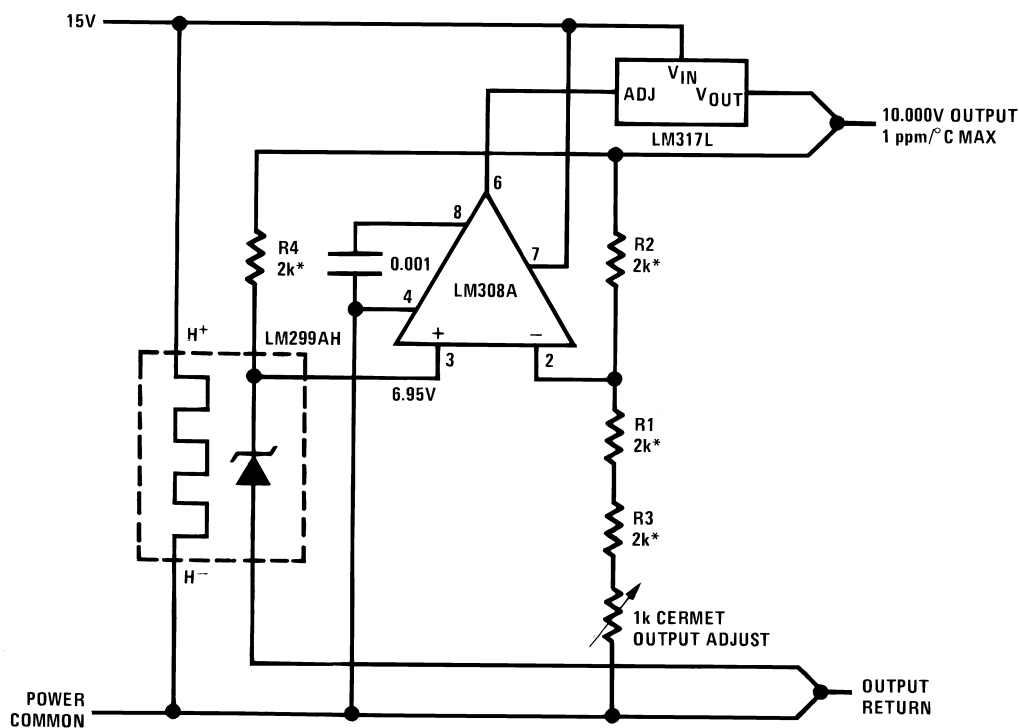
Precision Reference with Short-Circuit Proof Output
