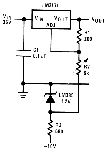
0V–30V Regulator
