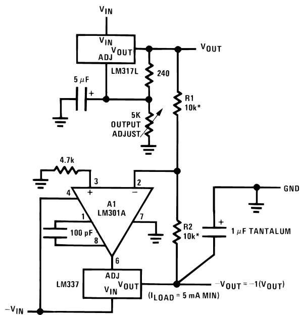
Tracking Regulator
