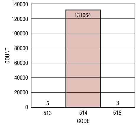
LTC2234: Noise Histogram
