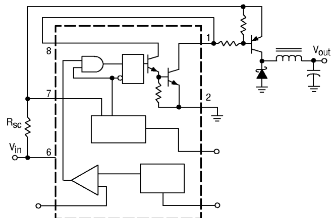
10b. External PNP Saturated Switch
