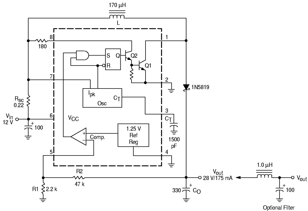
Figure 7. Step-Up Converter
