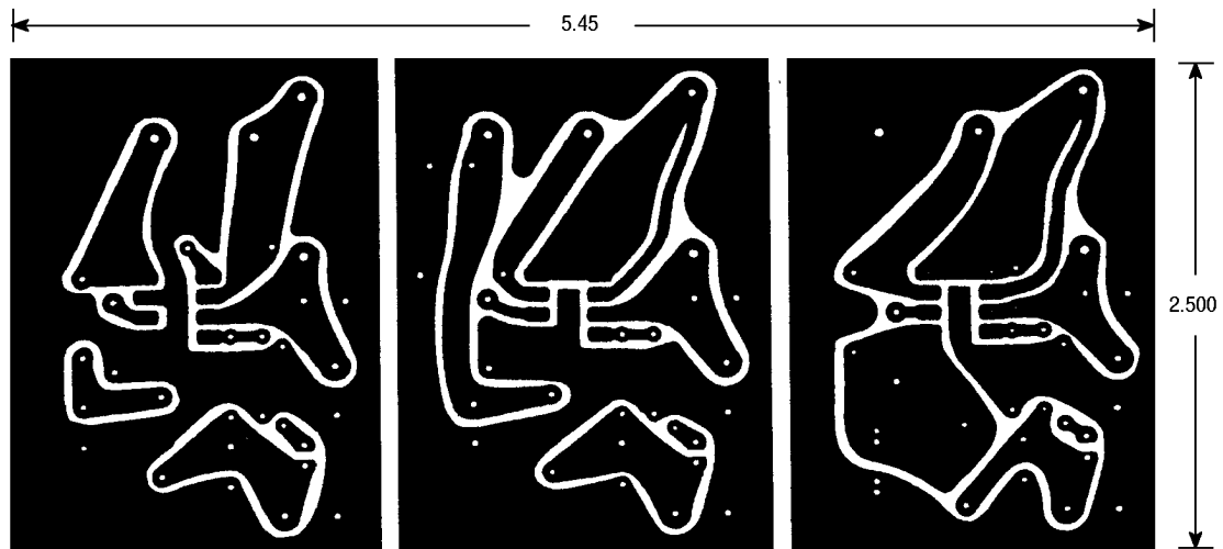
Figure 13. Printed Circuit Board and Component Layout (Circuits of Figures 7, 9, 11)
