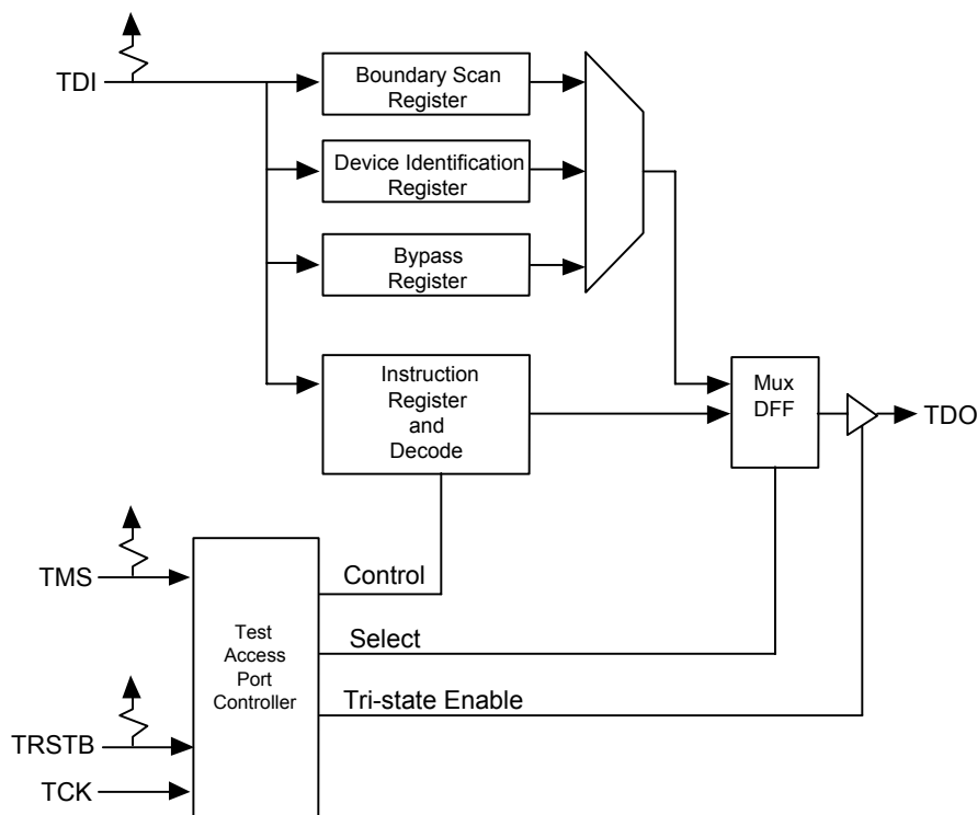
Figure 32 - Boundary Scan Architecture
