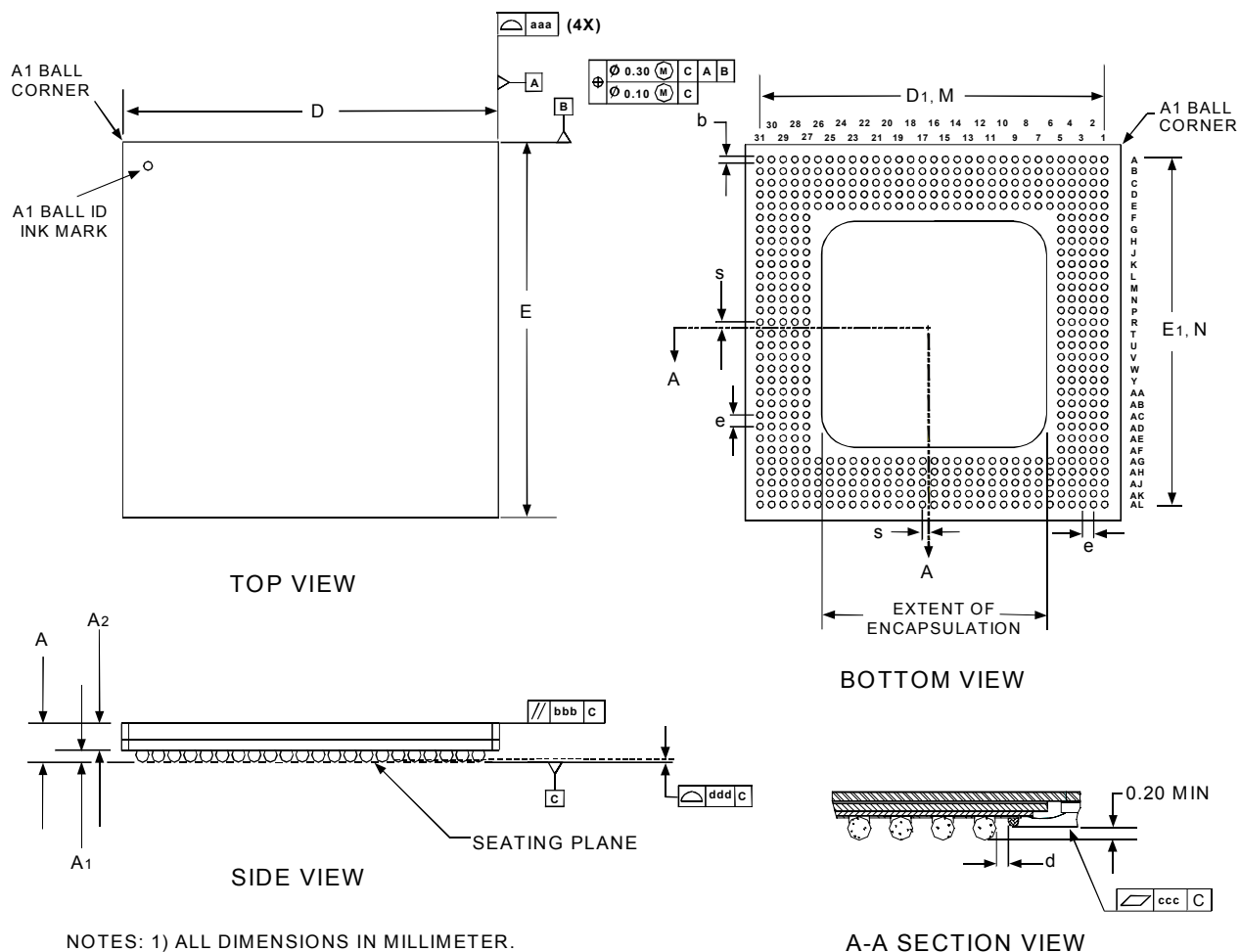
Figure 69 - 520 Pin Enhanced Ball Grid Array (SBGA)
