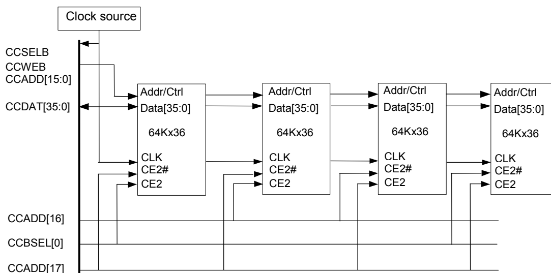
Figure 28 - 4 Bank Configuration for 8 MB of ZBT or Standard SSRAM
