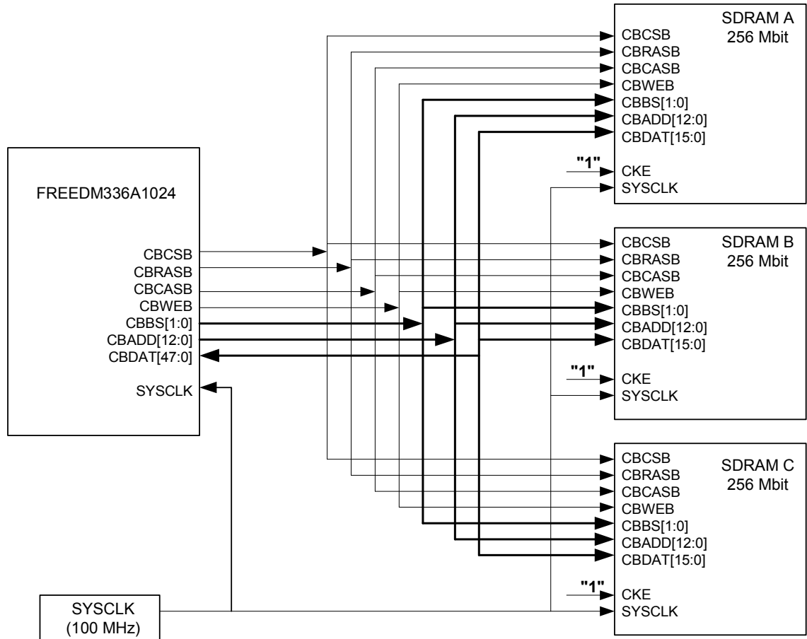
Figure 26 - DRAM configuration for the Chunk Buffer Interface
