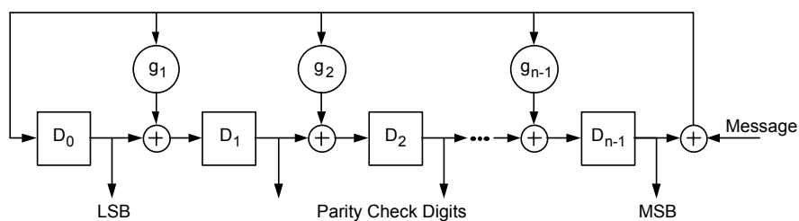
Figure 16 - CRC Generator
