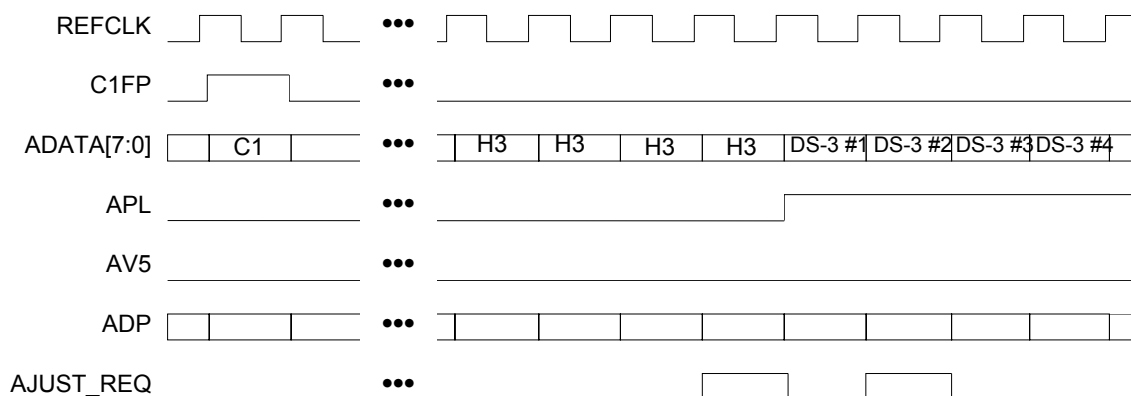
Figure 36 - DS3 Add Bus Adjustment Request Functional Timing
