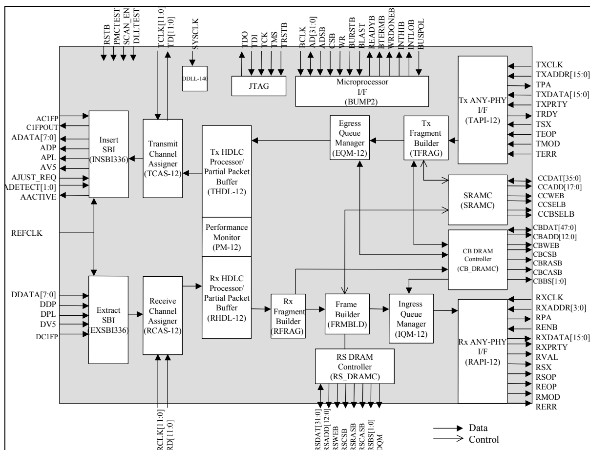
Figure 2 - The block diagram of FREEDM-336A1024
