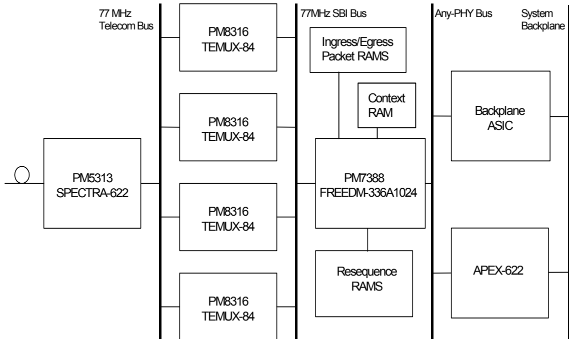
Figure 1 - An OC-12 access card for a router
