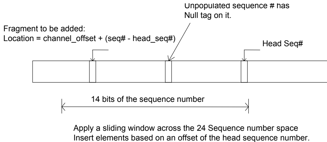
Figure 21 - The 14-bit sliding window used for re-sequencing
