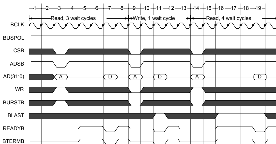
Figure 56 - Read and Write to non-burstable register space
