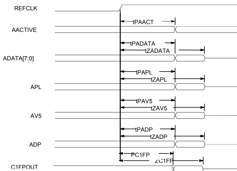
Figure 61 - SBI336 Add Bus Output Interface Timing
