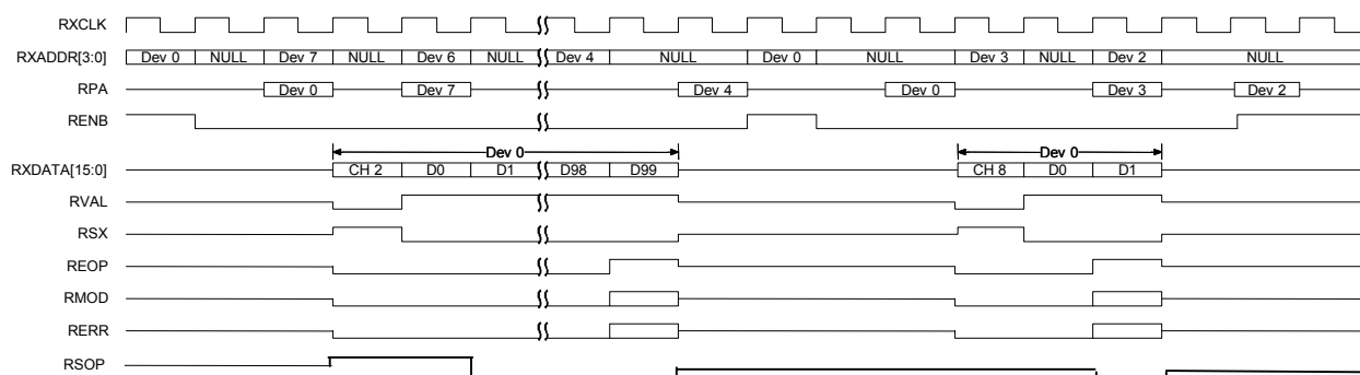
Figure 40 - Receive APPI Timing (Auto Deselection)
