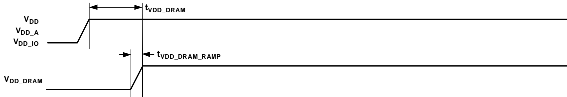
Figure 7. Power-Up Timing
